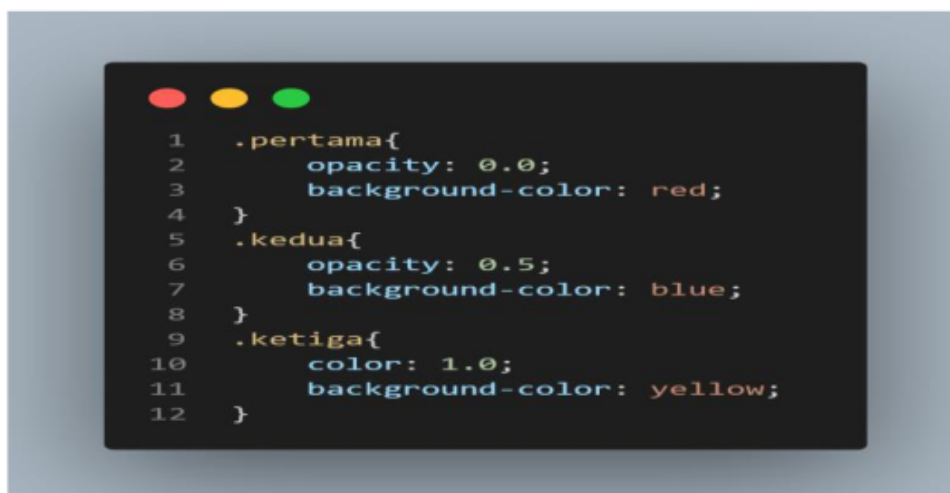
Gambar 3.56 Script css opacity
