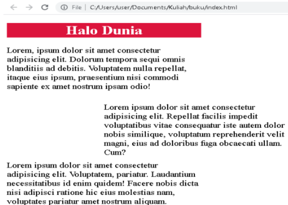
Gambar 3.83 Hasil script relative position
