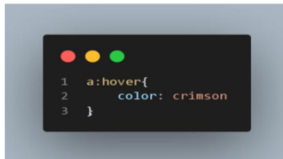
Gambar 3.29 Script css pseudo selector
