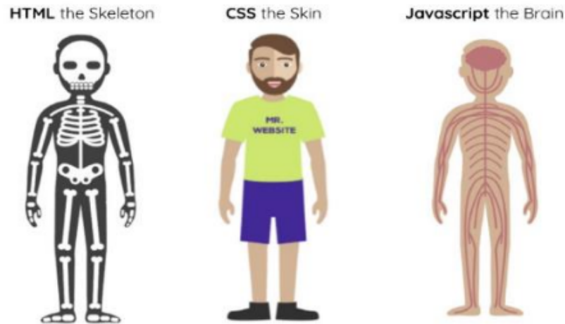
Gambar 1.2 anatomi website
