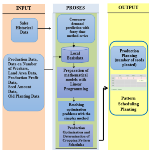
Fig. 1. Information system framework
