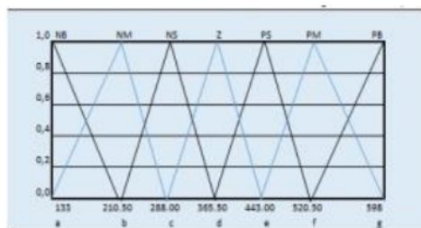
Fig. 2. Universe of discourse
