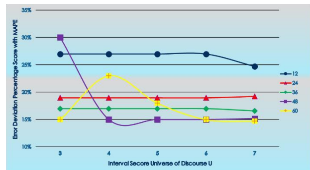
Fig 3. Error deviation score with MAPE
