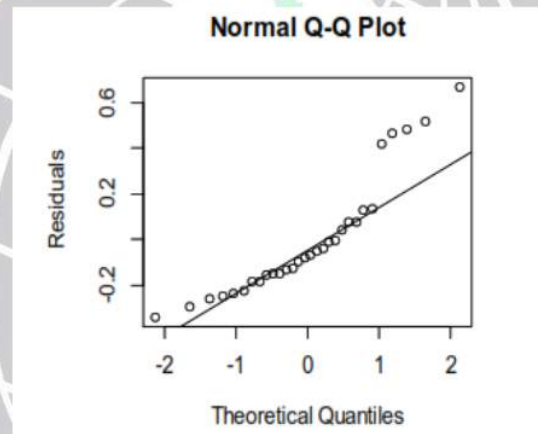
Gambar 4. Plot Probabilitas Normal
