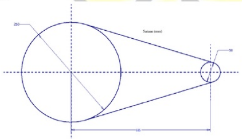
Gambar 3. Dimensi driver pulley , belt dan driven pulley
