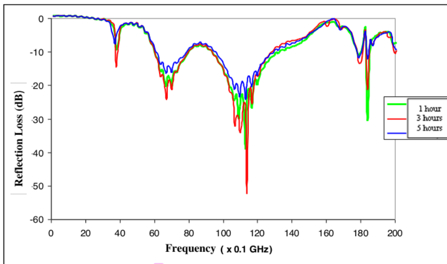
Figure 3. Characteristics of the microwave absorption properties of the samples sintered at 300°C with variations in holding time for 1 hour, 3 hours, and 5 hours.
