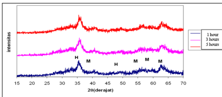
Figure 1. X-ray diffraction patterns of samples sintered at 300°C with various holding times of 1 hour, 3 hours and 5 hours.
