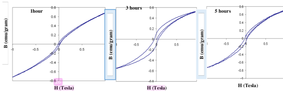
Figure 2. Hysteresis curve of the BaFe 12 O 19 which was sintered at 300 0 C
