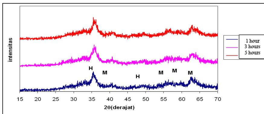
Figure 1. X-ray diffraction patterns of samples sintered at 300 0 C with various holding times of 1 hour, 3 hours and 5 hours.
