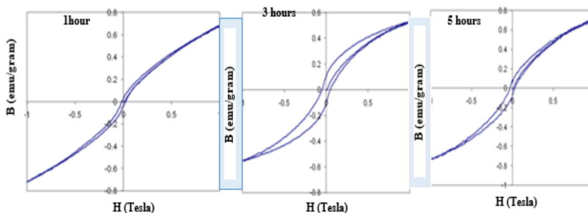
Figure 2. Hysteresis curve of the BaFe 12 O 19 which was sintered at 300 0 C
