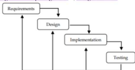
Gambar 4. Alur Penelitian
