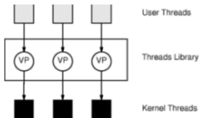
1:1 Threads Model
