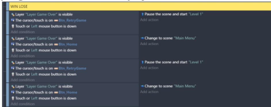
Gambar 7. 86 Duplikasi Program Layer Game Over
