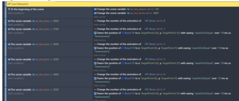
Gambar 5. 52 Hasil Akhir Program HP_Boss
