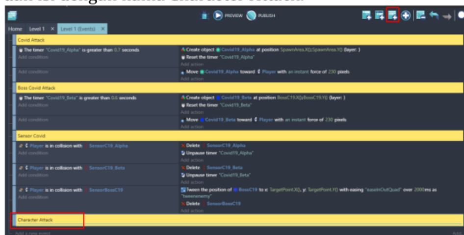
Gambar 3. 11 Menambahkan Comment Character Attack
