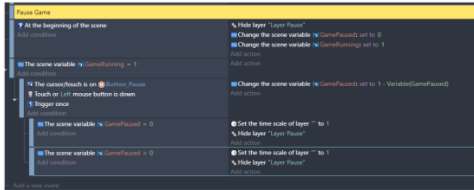
Gambar 4. 50 Duplikasi Program The Scene Variable GamePaused
