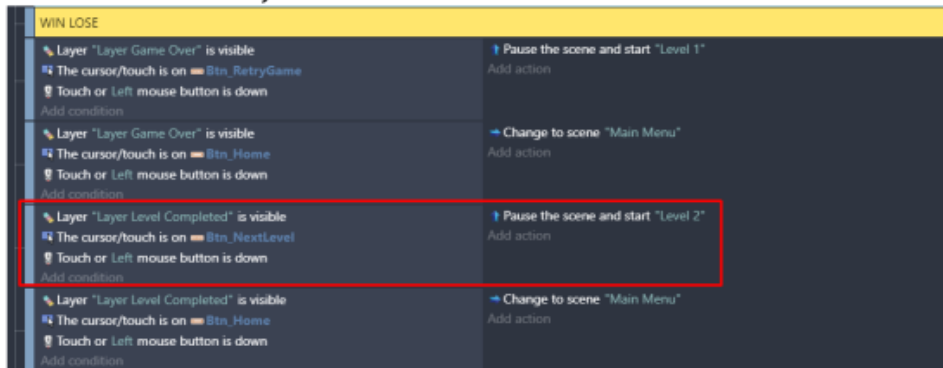
Gambar 7. 88 Mengubah Objek Layer Level Completed
