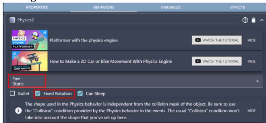
Gambar 1. 37 Mengatur Behaviors Physics engine 2.0
