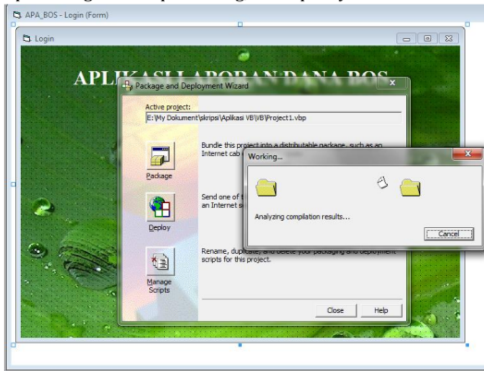
Gambar 50. Proses compiler
