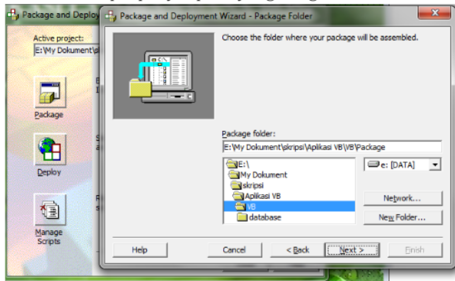
Gambar 52. Package Folder
