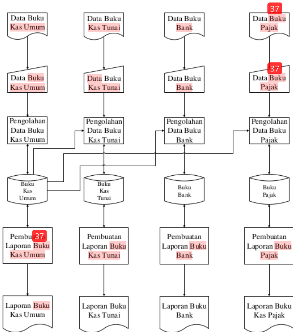
Gambar 6. Flowchart Sistem
