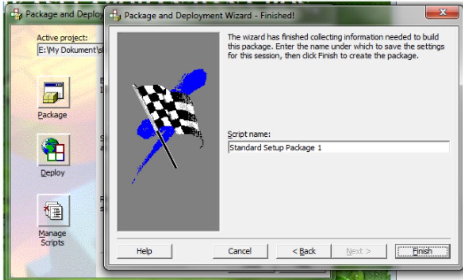
Gambar 58. Jendela Finished
