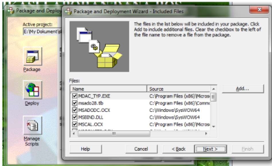
Gambar 53. Included Files
