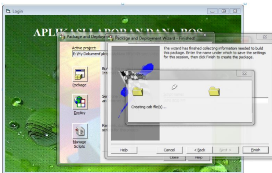
Gambar 59. Proses finished
