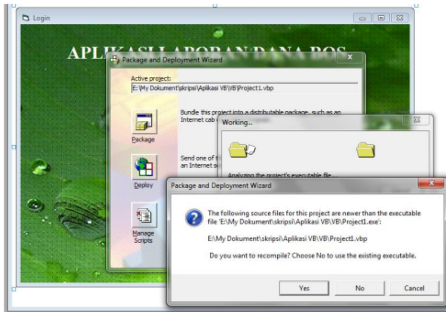
Gambar 49. Dialog recompiler
