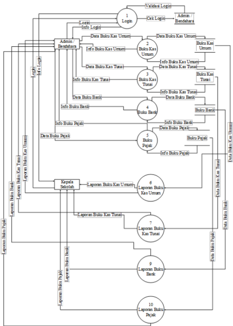
Gambar 3. DFD Level 1
