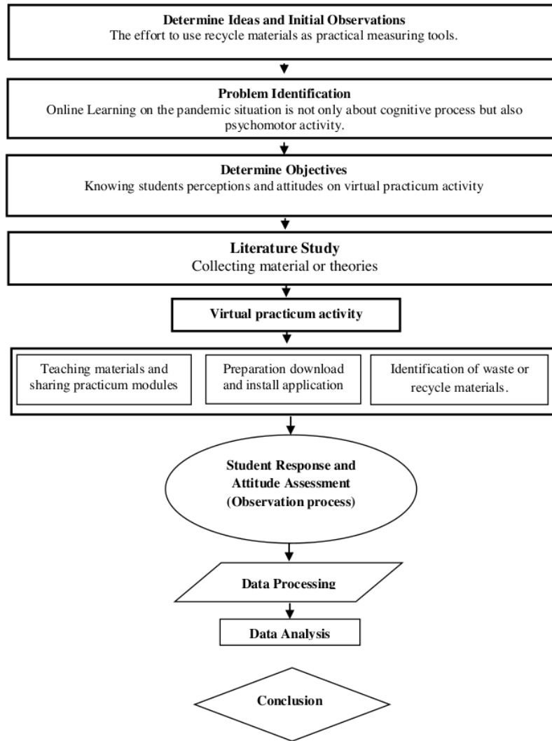
Figure 1. Research Flowchart
