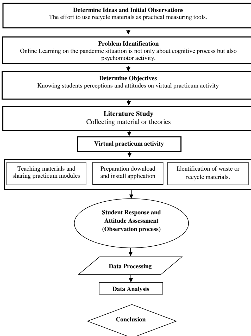
Figure 1. Research Flowchart
