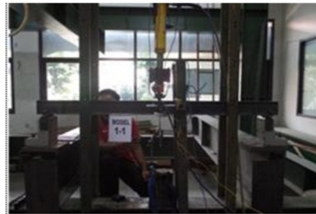
Gambar 10. Setting up pengujian
